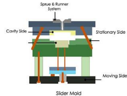
Two plate mold
