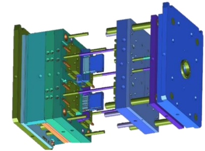
Three plate mold
